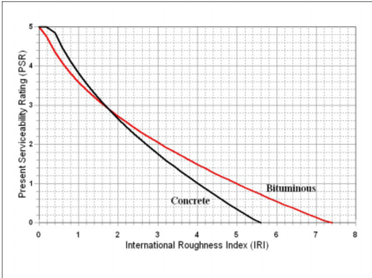
Figure 4. Graph for converting IRI to PSR (based on the 1997 rating panel)
