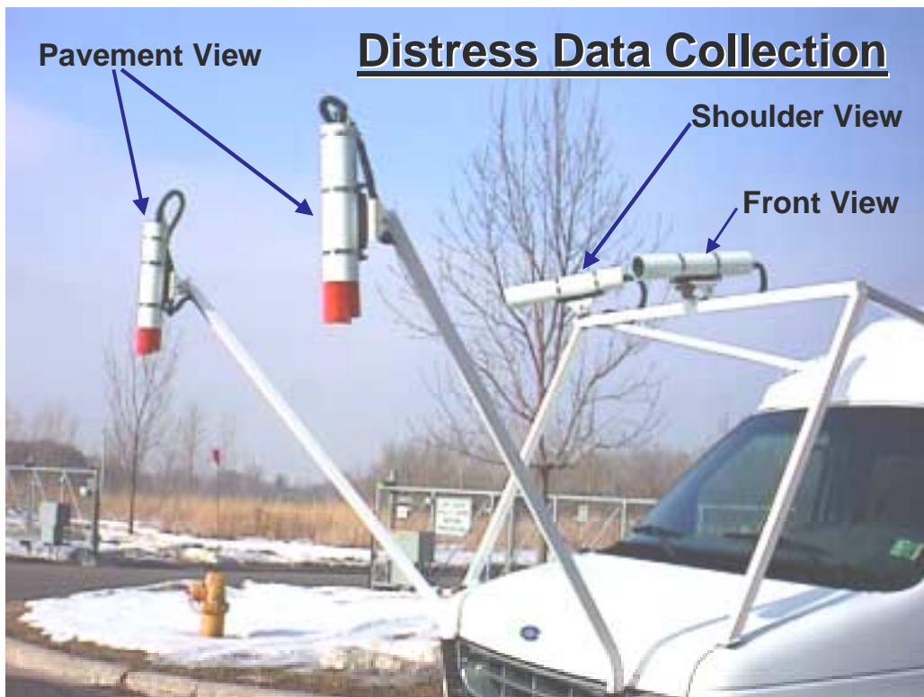
Figure 3. Close-up of cameras used to record pavement distress.
