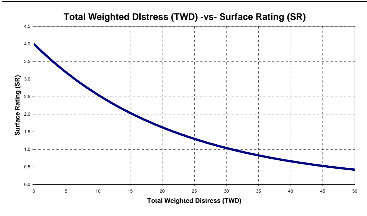
Figure 6. Chart for calculating Surface Rating (SR) from the Total Weighted Distress (TWD)
