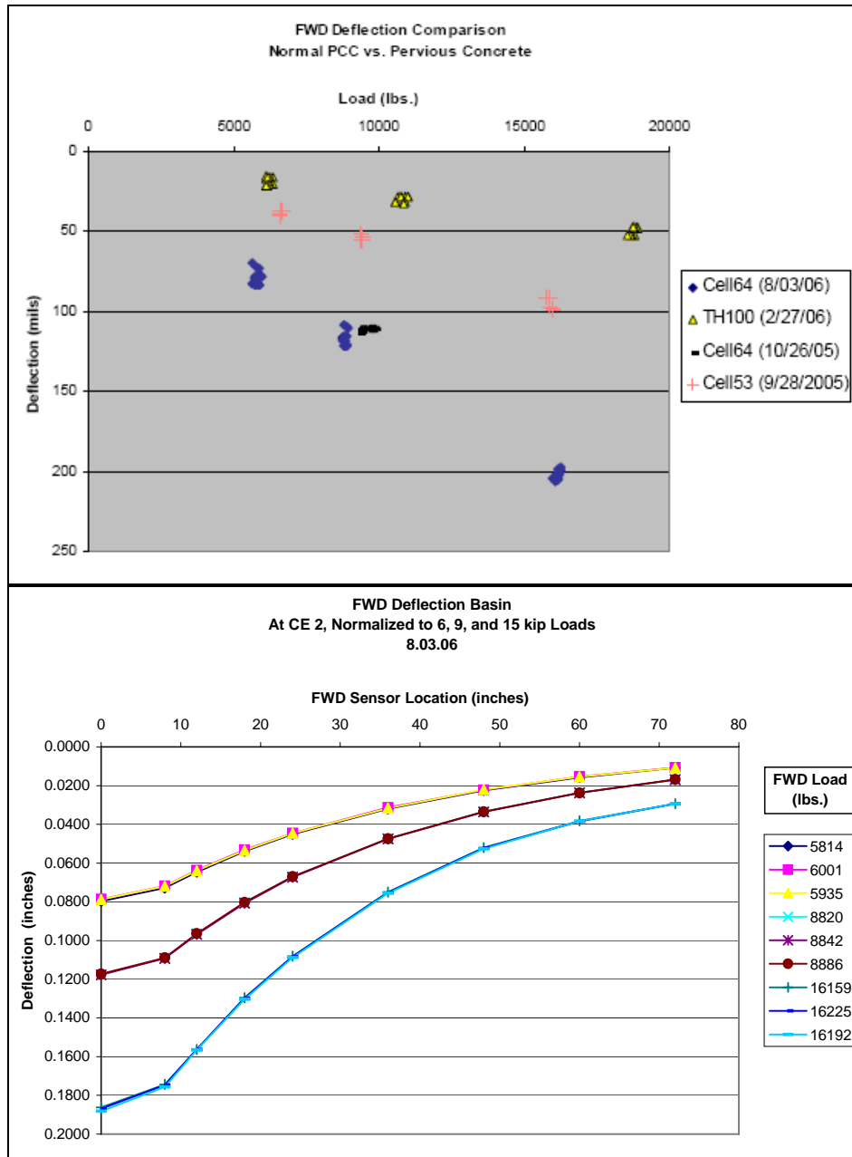
FIGURE 4 Comparison of maximum FWD in normal PCC and pervious PCC and pervious PCC normalized FWD deflection basin.
