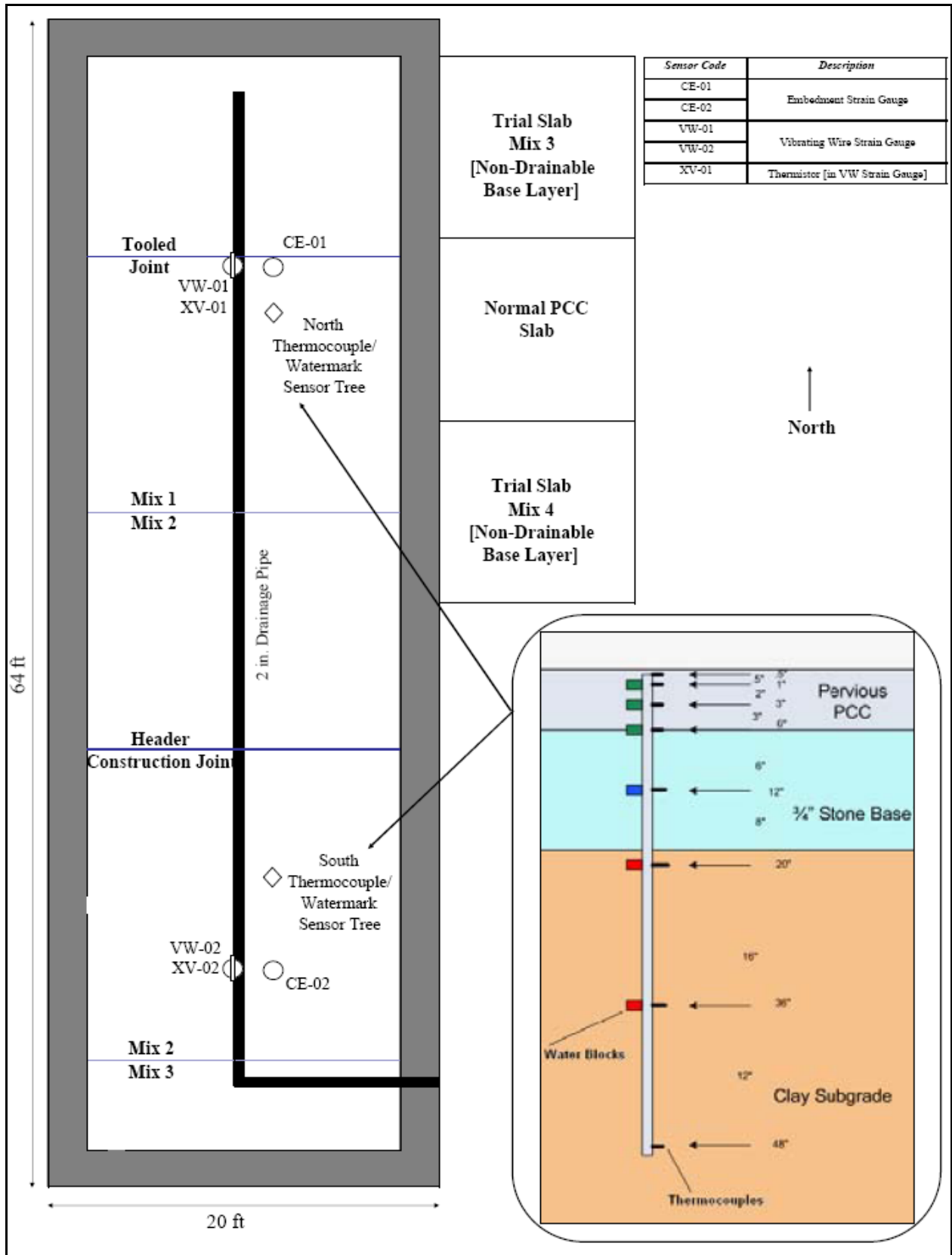
FIGURE 1 Plan and elevation views of test cell and instrumentation.
