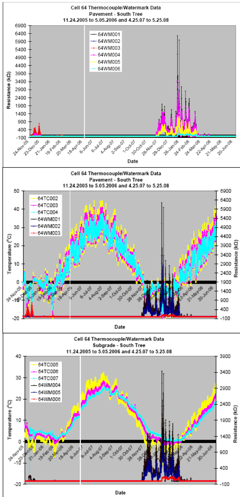
FIGURE 2 Top: water mark, middle: water mark and thermocouple (pavement), bottom: thermocouple and watermark (subgrade).
