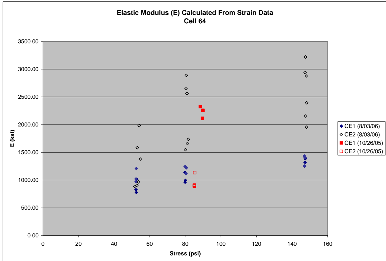
FIGURE 5 Elastic Modulus Calculated From FWD Strain Data.
